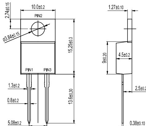
TO-220AC DR16XX
